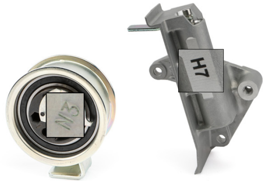
Photo 1: Tensioner pulley 531 0396 20 with vibration damper 533 0039 10
